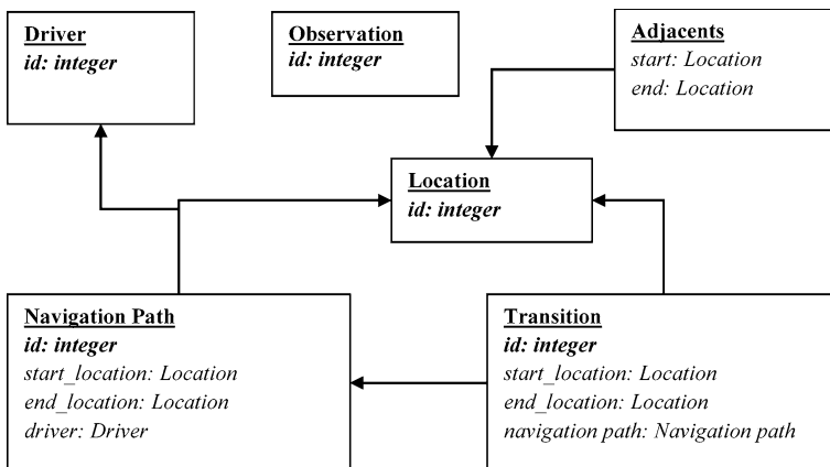
Fig. 11 Database schema showing major links
