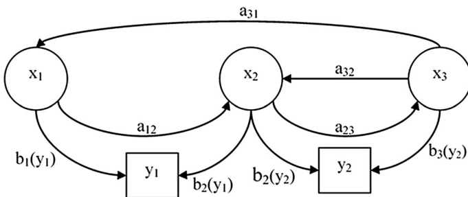
Fig. 1 Hidden Markov model
