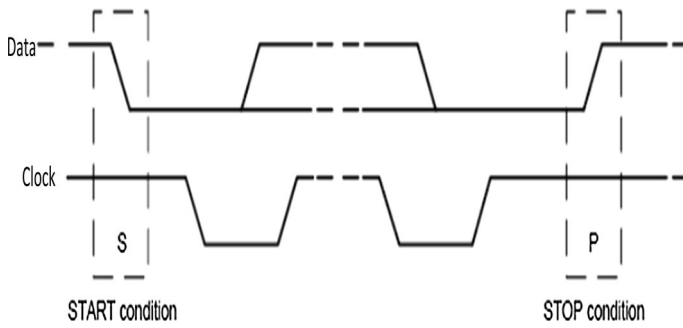
Fig. 9 I 2 C protocol start and stop conditions
