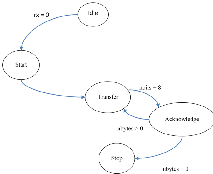
Fig. 9 I 2 C protocol start and stop conditions
