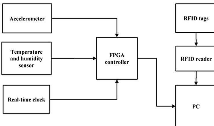
Fig. 4 Detailed hardware design of implemented system
