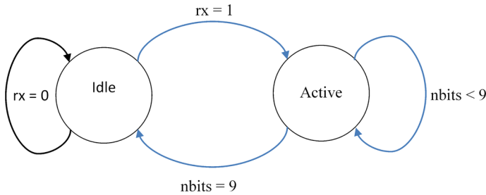
Fig. 8 UART reception FSM
