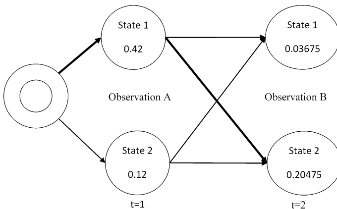
Fig. 13 Viterbi algorithm visualizer
