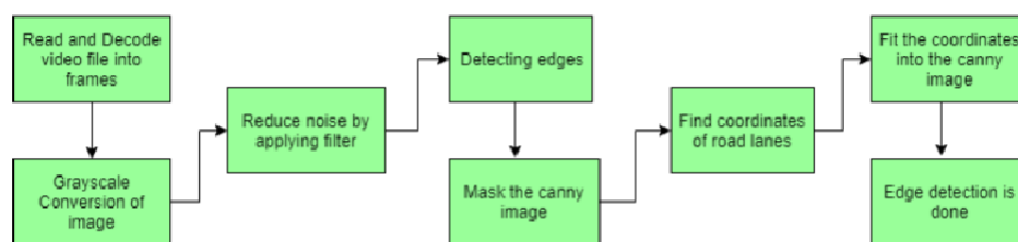
Flowchart Of Lane Detection
