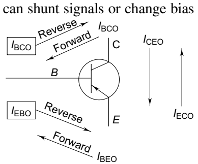
Fig. 2.42 Leakage paths in a transistor
