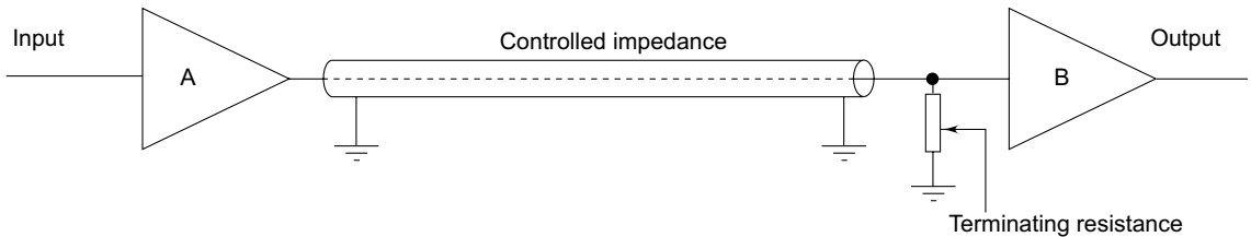
Fig. 4.17 Single-ended PCB trace
