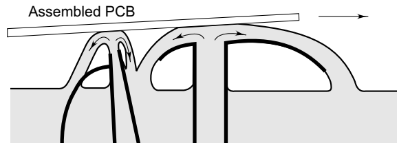
Fig. 13.30 Schematic of a dual wave soldering machine—turbulent first wave and a smooth second wave
