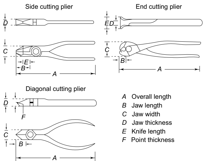
Fig. 13.9 Side cutter
