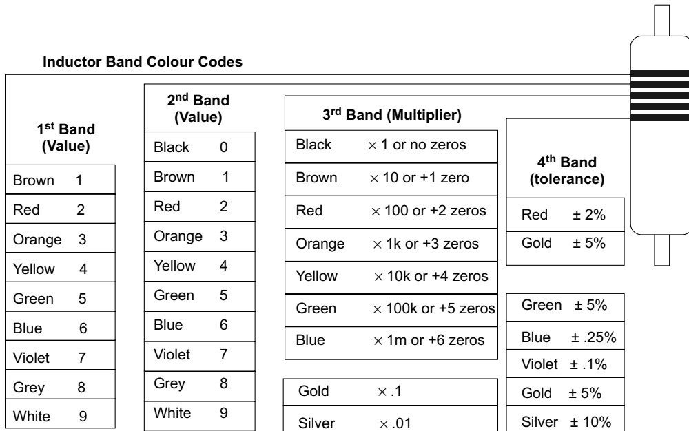
Fig. 2.27 Colour code for inductors
