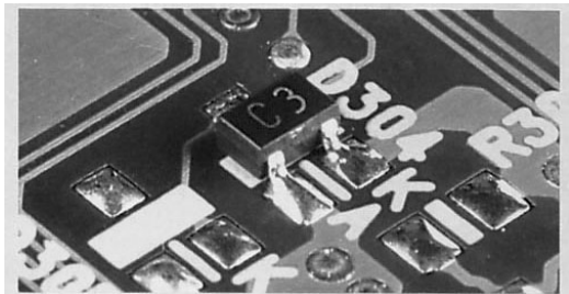
d. Insufficient solder
