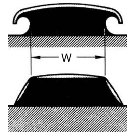
Fig. 14.19 Conductor width
