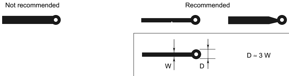
Fig. 5.13 Solder pad diameter and conductor width
