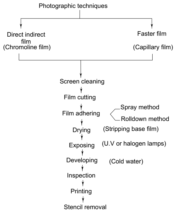
Fig. 7.9 Flow chart for photographic technique for image transfer
