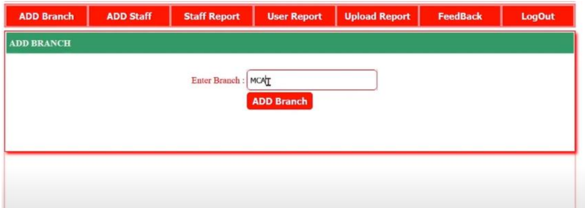
Figure 16 Project Snap4
