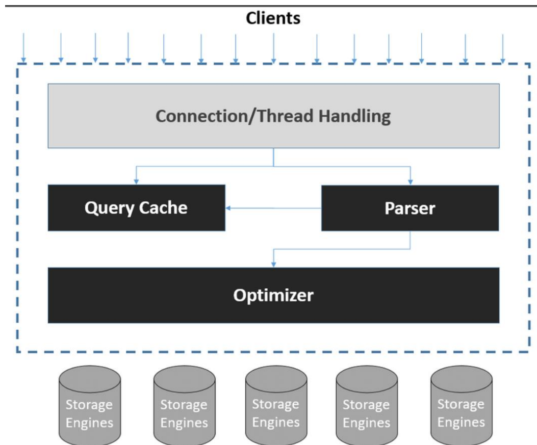
Figure 7: Mysql Architecture
