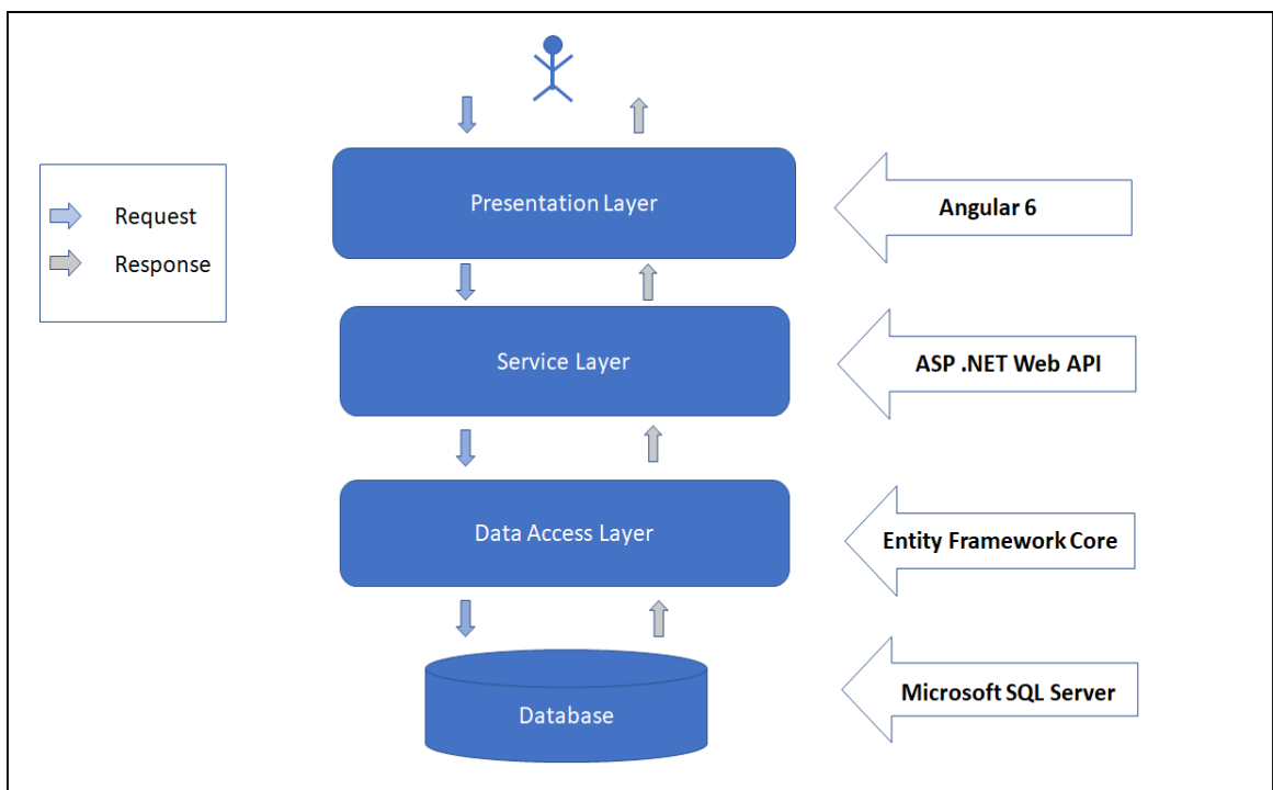
Figure 10: Architecture
