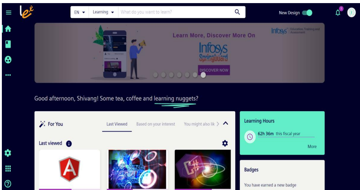
Figure 6: Lex Portal
