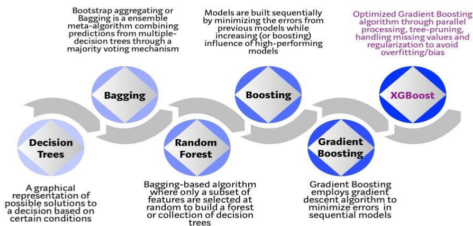
FIG.8 XG Boost diagram
