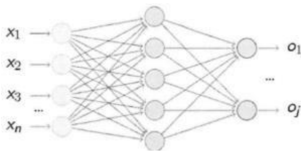
Figure 1 Schematic diagram of a fully connected network h_1 W_1 x b_1; z act(h_1) ; o W_2 z b_2
