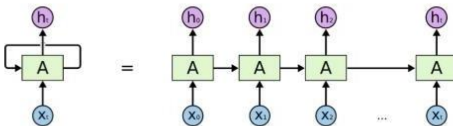
Figure 3 Structure form of standard RNN
